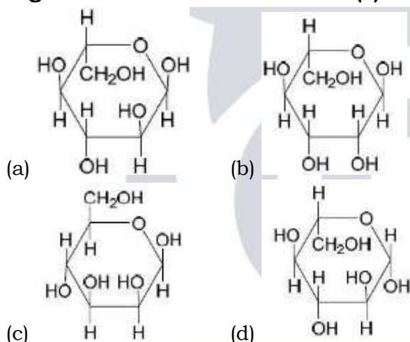
D-glucose
