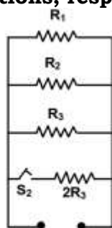
Circuit-2
