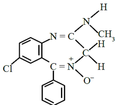
Chlordiazepoxide
