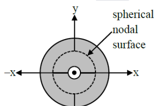
Figure 1. electron probability density for 2
