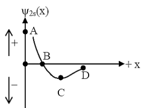
Figure 2. wave function for 2 s orbital
